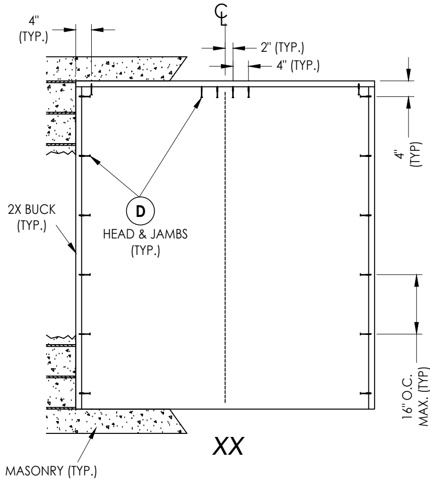
XX BUCK ANCHORING
