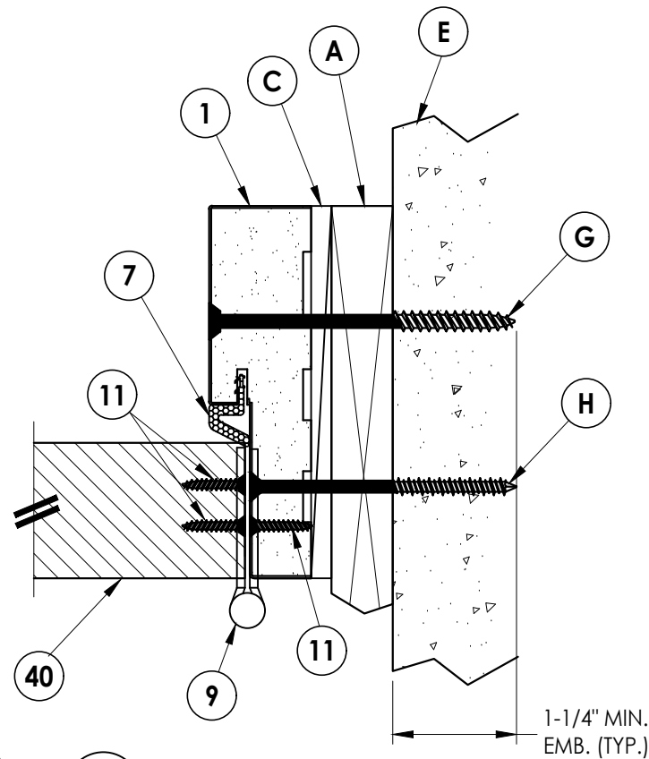
7 3 HORIZONTAL CROSS SECTION Shown w/1X sub-buck
