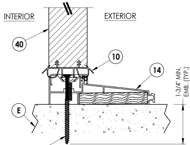
3 3 HORIZONTAL CROSS SECTION Inswing threshold
