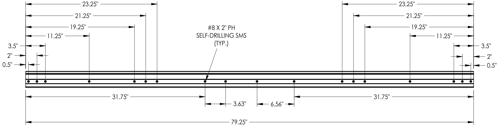
ASTRAGAL SCREW LOCATIONS
